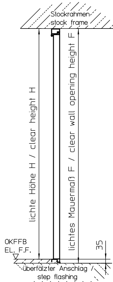
Z-Zarge Z-frame
