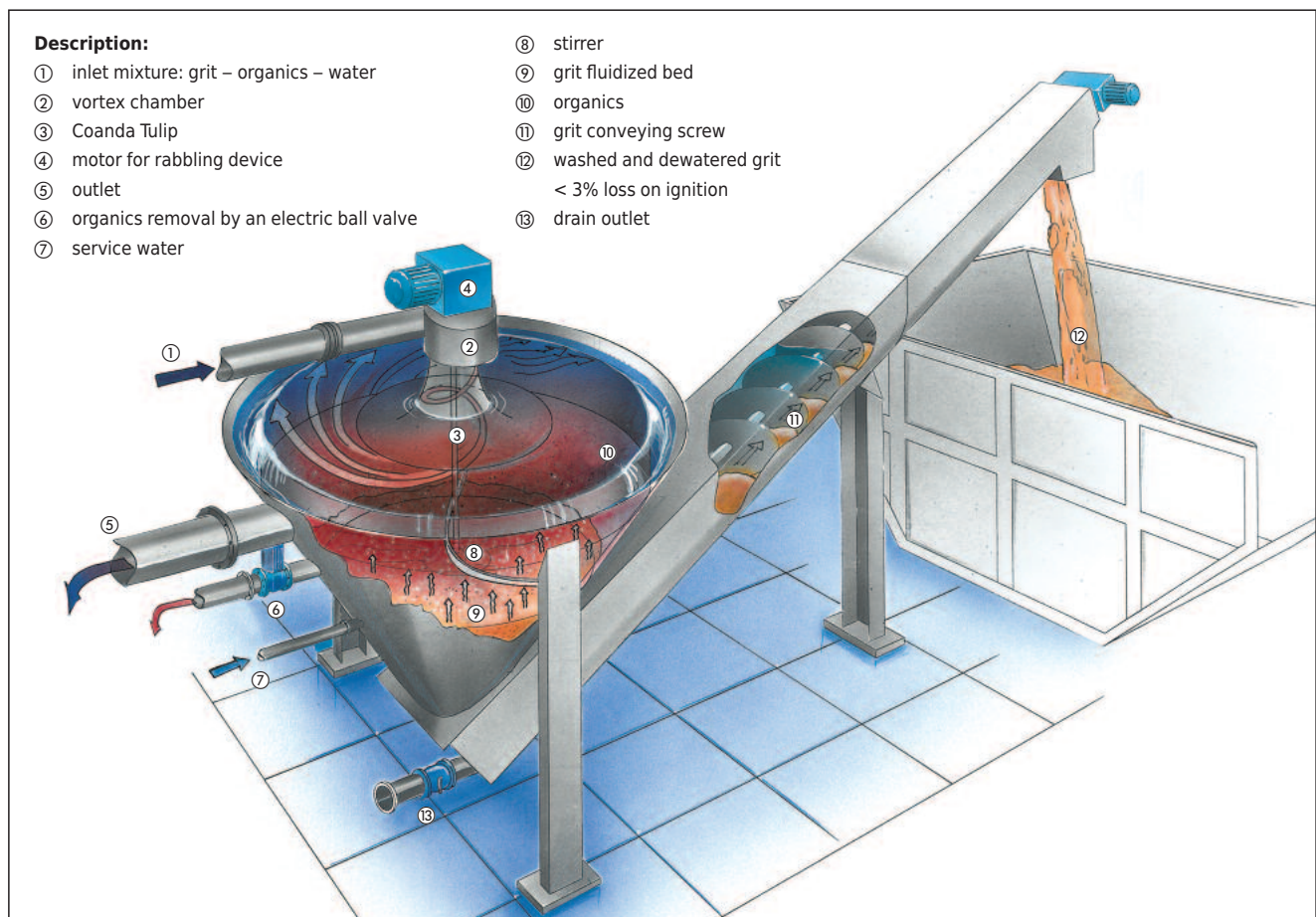
Flow diagram of a HUBER Coanda Grit Washer RoSF4
