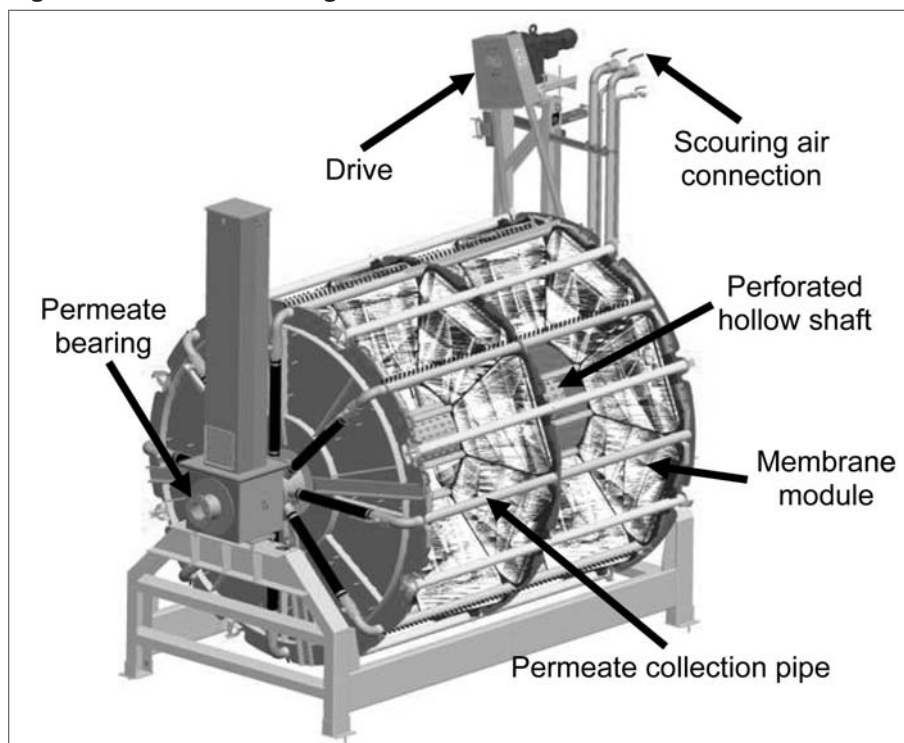
Figure 2. Detailed Drawing of a Vacuum Rotation Membrane Unit
